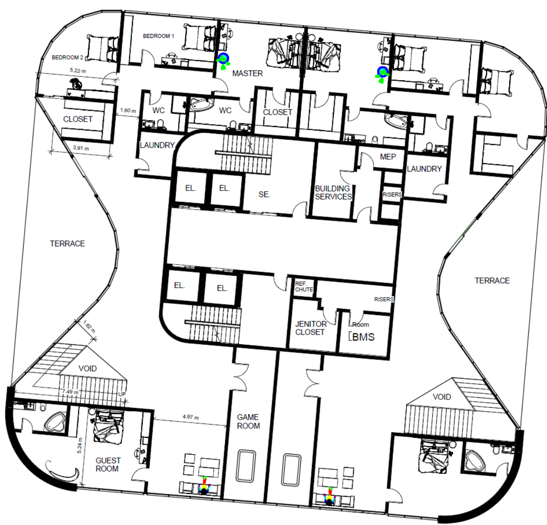
Pent House 2nd Floor Plan
